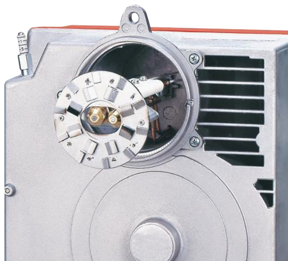
Combustion head (RG5D)
